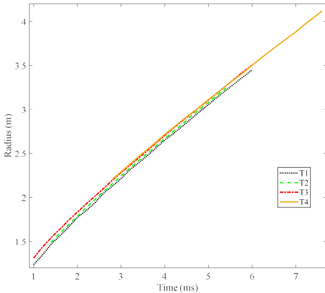
Fig. 4. Blast wave position-time graph for each test.
