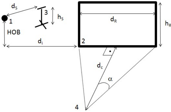
Fig. 2. Tests setup presenting the positioning of the explosive charge (1), the wood structure for image calibration (2), the pressure gauges (3) and the high-speed camera (4).
