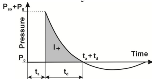
Fig. 1. Pressure-time profile generated by the passage of a blast wave through air.
